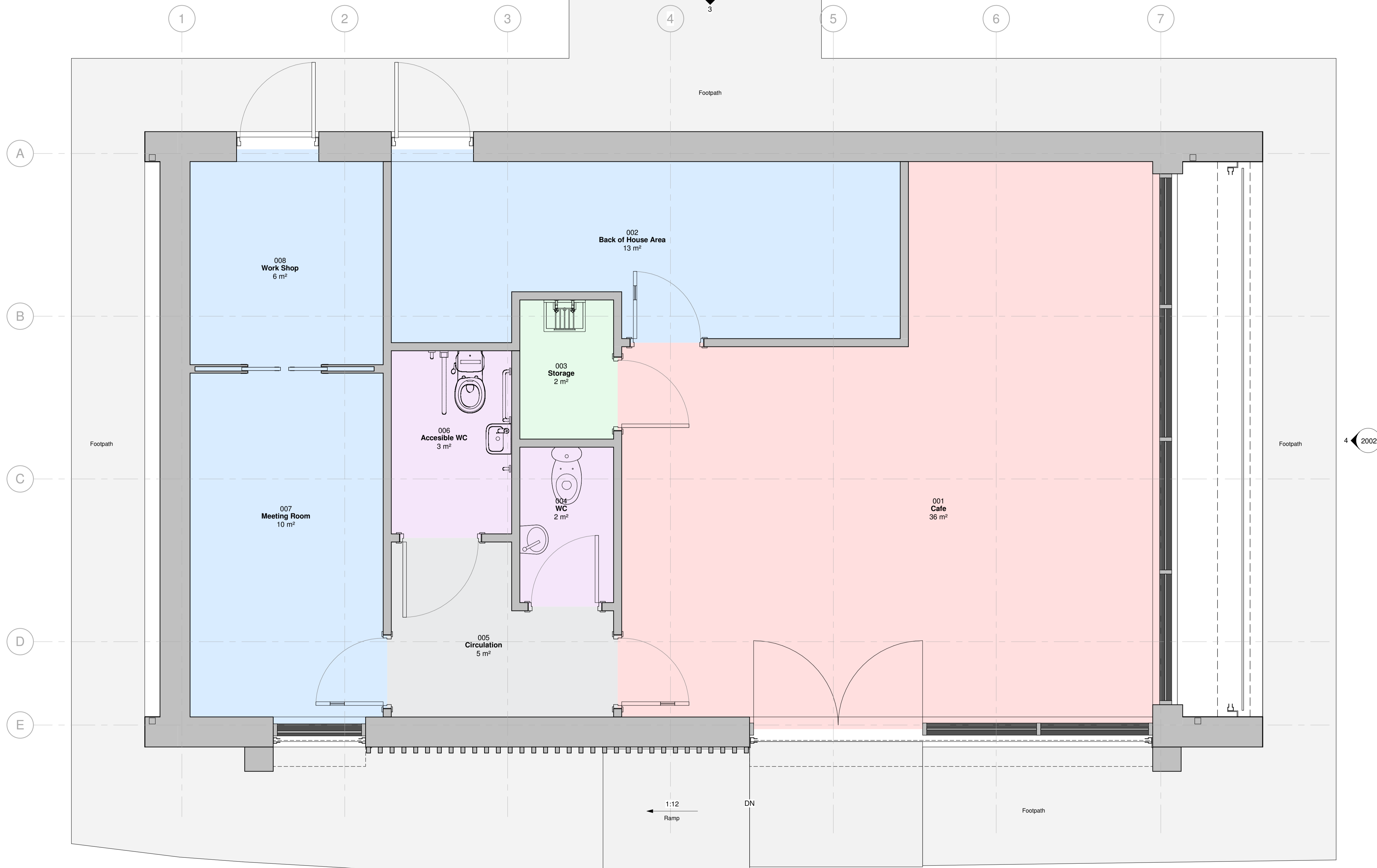
1 GA_Plan_Ground_Floor 1:25
